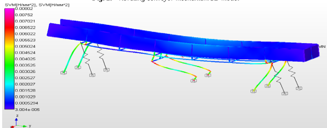
Fig. 2. Vibrating conveyor mechanism 3D model
