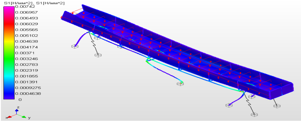
Fig. 7. Computed plot of the stress-strain state \tau_{YZ} .
